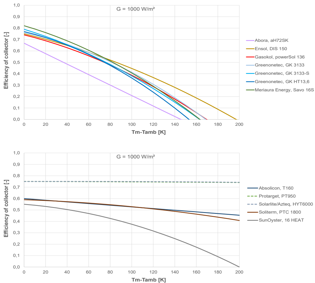
Figure 1: Selected efficiency curves for flat-plate collectors (above) and parabolic trough collectors (below). Solid lines are based on Solar Keymark certificates and dotted lines are based on manufacturer information. Dotted curves for Protargel and Solarlite/ Azteq are overlapping
